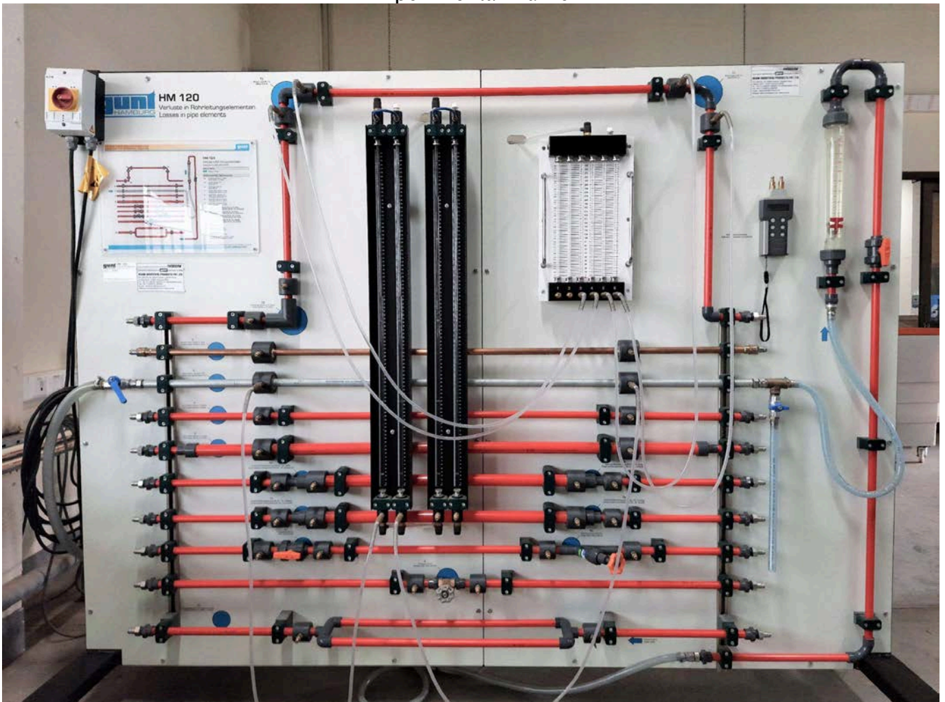
Pipe network experiment.
